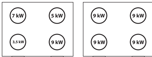
Figure 6. Location of burners in the four-burner stove (schematically)
