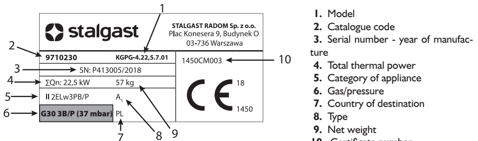
Figure 17. Example of the nameplate
